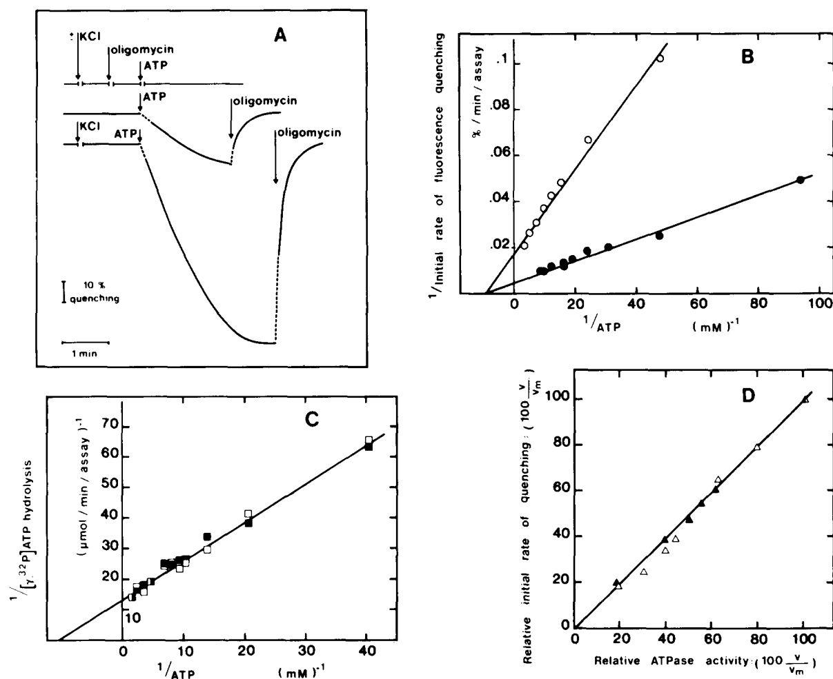
Fig. 3. Correlation between ATP hydrolysis and fluorescence quenching of ACMA in the ATPase-ATP synthase complex. The complex (0.11 mg) was preincubated for 1 min in the medium containing valinomycin as described in Materials and Methods in the presence (●, ■, ▲) or in the absence (○, □, △) of 50 mM KCl. The reaction was initiated by addition of ATP at the indicated concentrations. To measure the rate of [\gamma\text{-}^{32}\text{P}]\text{ATP} hydrolysis, the reaction was stopped after 15 s by introduction of the sample in the ^{32}\text{P}_i extraction mixture. The ^{32}\text{P}_i liberated was counted as previously described [11]. (A) Fluorescence quenching of ACMA induced by 0.04 mM ATP, effect of KCl and oligomycin (5 \mu\text{g}/\text{assay} ); (B) effect of ATP concentration on the initial rate of the ATP-dependent fluorescence quenching of ACMA in the presence (●—●) or in the absence (○—○) of KCl; (C) effects of [\gamma\text{-}^{32}\text{P}]\text{ATP} concentration ( 7 \cdot 10^3 cpm/nmol) on the rate of [\gamma\text{-}^{32}\text{P}]\text{ATP} hydrolysis in the presence (■—■) or in the absence (□—□) of KCl; (D) plot of relative initial rate of fluorescence quenching of ACMA versus initial rate of [\gamma\text{-}^{32}\text{P}]\text{ATP} hydrolysis in the presence (▲) or in the absence (△) of KCl.
