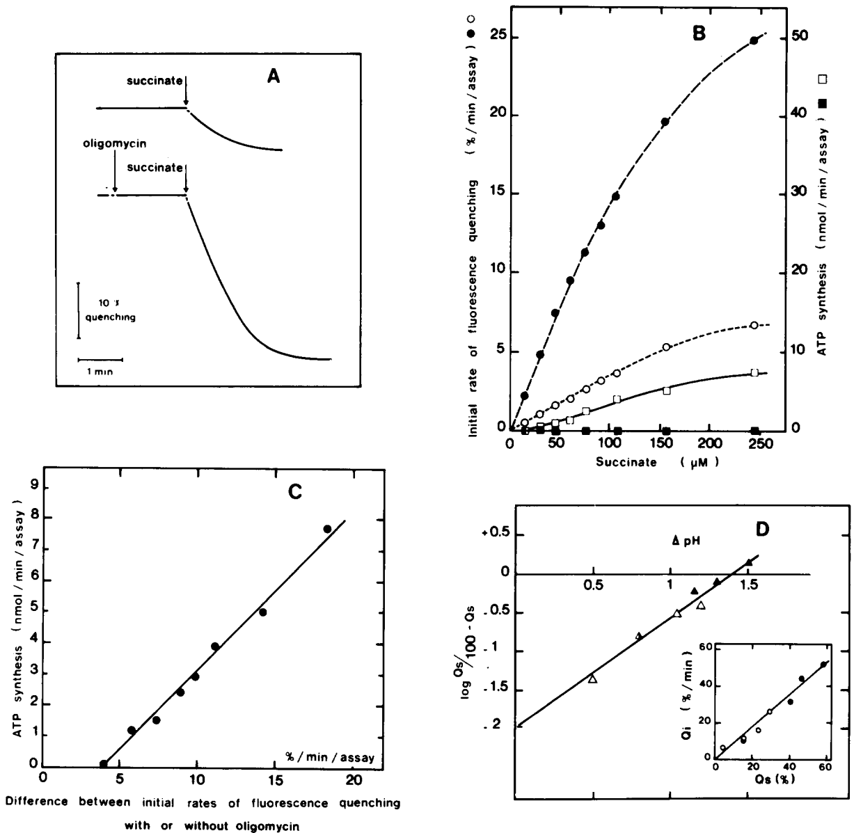
Fig. 5. Correlation between net ATP synthesis and quenching of fluorescence of ACMA in inverted submitochondrial particles oxidizing succinate. Relation between \Delta \text{pH} and quenching. Inverted submitochondrial particles (0.45 mg) were preincubated for 1 min in the medium described in Materials and Methods, except that glucose (10 mM), ADP (5 mM), potassium phosphate (20 mM) (final concentrations) were added. KCl was also added to match the final \text{K}^+ concentration of 50 mM. 30 units hexokinase were present in each assay (2 ml). When indicated, oligomycin (5 \mu\text{g} /assay) was present. The reaction was initiated by addition of succinate at the indicated concentrations, and stopped 30 s later for [\gamma\text{-}^{32}\text{P}]\text{ATP} synthesis measurements (see Materials and Methods). The specific radioactivity of ^{32}\text{P}_i was 18 \cdot 10^3 cpm/nmol. (A) Fluorescence quenching of ACMA induced by 0.15 mM succinate in the presence or in the absence of oligomycin; (B) effect of succinate concentration on the initial rate of [\gamma\text{-}^{32}\text{P}]\text{ATP} synthesis and of the succinate dependent fluorescence quenching of ACMA in the presence (●, ■) or in the absence (○, □) of oligomycin; (C) [\gamma\text{-}^{32}\text{P}]\text{ATP} synthesis as a function of the difference between the initial rates of fluorescence quenching of ACMA obtained for each concentration of succinate in the presence of oligomycin and that obtained in the absence of oligomycin (data from (B)); (D) relation between \Delta \text{pH} and fluorescence quenching of ACMA induced by addition of succinate at concentrations ranging from 0.012–0.15 mM in the presence (▲) or in the absence (△) of oligomycin. The \Delta \text{pH} was estimated as described in Materials and Methods. Q_s is the quenching at the steady state. Insert: initial rate of fluorescence quenching ( Q_i ) as a function of quenching at the steady state ( Q_s ).
