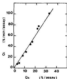
Fig. 2. Correlation between initial rate of ACMA fluorescence quenching ( Q_i ) and ACMA fluorescence quenching at steady state ( Q_s ) when energization was induced by various ATP concentrations. Conditions as in Fig. 1A except that the ATP concentration varied from 0.02–0.24 mM.
