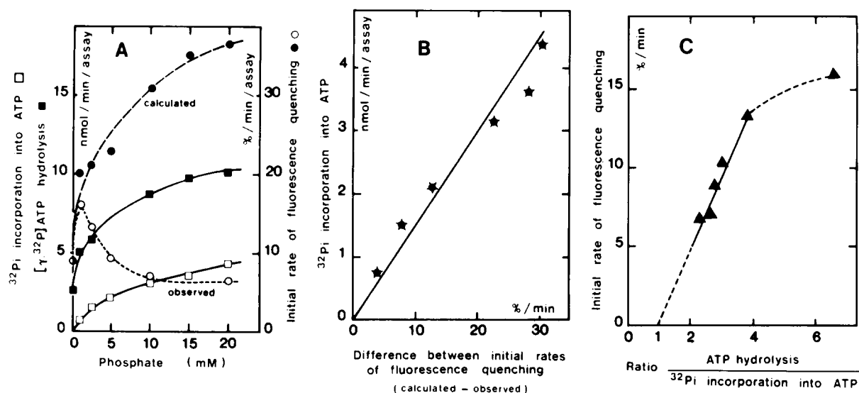
Fig. 4. Correlation between the rate of ^{32}\text{P}_i incorporation into ATP and relative disappearance of initial rate of fluorescence quenching of ACMA in ATPase-ATP synthase complex. The complex (0.11 mg) was preincubated for 1 min in the medium described in Materials and Methods, except that 0.5 mM ADP and potassium phosphate at the indicated concentration were added. The \text{K}^+ concentration was maintained at 50 mM in each assay by an adequate KCl addition. The reaction was initiated with 212 \mu\text{M} ATP and stopped 30 s later to measure the amount of [\gamma\text{-}^{32}\text{P}]\text{ATP} hydrolyzed or ^{32}\text{P}_i incorporated into ATP (ATP- ^{32}\text{P}_i exchange) as previously described [11]. (A) Effect of phosphate concentration on the initial rate of [\gamma\text{-}^{32}\text{P}]\text{ATP} hydrolysis (■—■), ^{32}\text{P}_i incorporation into ATP (□—□) and fluorescence quenching of ACMA observed (○—○) or calculated (●—●). Calculated quenching for each \text{P}_i concentration: Q_p = H_p(Q_0/H_0) , where H_p is the rate of ATP hydrolysis at the indicated \text{P}_i concentration, Q_0 and H_0 are quenching and hydrolysis at [\text{P}_i] = 0 . The specific radioactivity used for the [\gamma\text{-}^{32}\text{P}]\text{ATP} hydrolysis measurements was 22 \cdot 10^3 cpm/nmol. For ATP- ^{32}\text{P}_i exchange activity, 50 \mu\text{Ci } ^{32}\text{P}_i was added in each sample. (B) ^{32}\text{P}_i incorporation into ATP as a function of the difference between the calculated and the observed initial rates of fluorescence quenching of ACMA obtained in (A). (C) Plot of the initial rate of fluorescence quenching of ACMA versus the ratio: ATP hydrolysis over ^{32}\text{P}_i incorporation into ATP. (The data are obtained from (A).)
