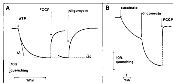
Fig. 1. Fluorescence quenching of ACMA induced by energization of inverted submitochondrial particles. (A) ATP-induced fluorescence quenching of ACMA. Inverted submitochondrial particles (0.26 mg) were preincubated for 1 min in the medium described in Materials and Methods, except that 50 mM KCl was present. The reaction was initiated with 0.05 mM ATP. FCCP (2.5 \mu M) or oligomycin (5 \mu g) were added when indicated. Q_i : initial rate of fluorescence quenching; Q_s : quenching of fluorescence at steady state. (B) Succinate-induced fluorescence quenching of ACMA. Inverted submitochondrial particles (0.26 mg) were preincubated for 1 min in the medium described in Material and Methods, except that 50 mM KCl/10 mM glucose/5 mM ADP/20 mM potassium phosphate/30 units hexokinase was present in each assay. The reaction was initiated by 0.3 mM succinate. Oligomycin (0.5 \mu g) and FCCP (2 \mu M) were added when indicated by the arrows.
